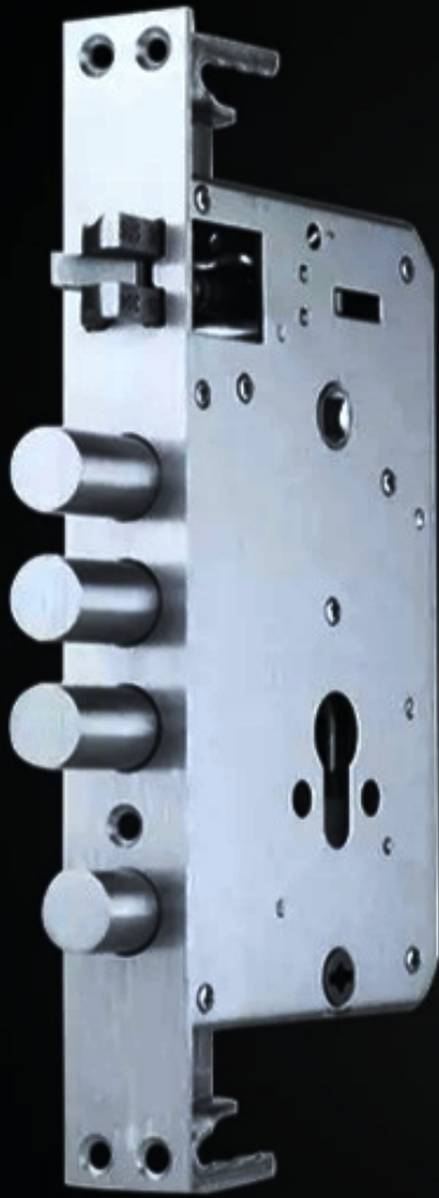
30×240 Cylindrical lock body
